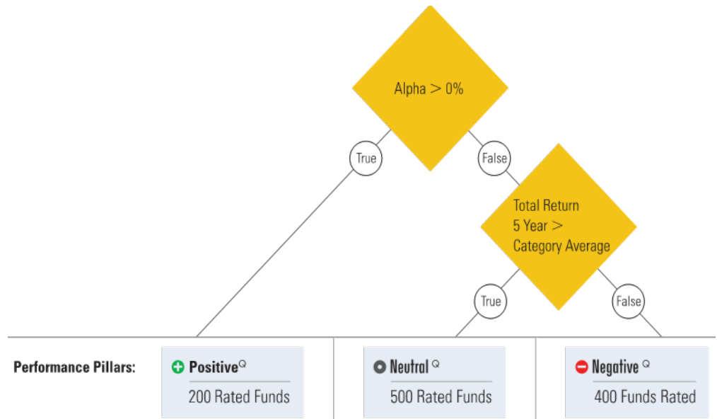
Exhibit 1 Sample Regression Tree With Dummy Data
